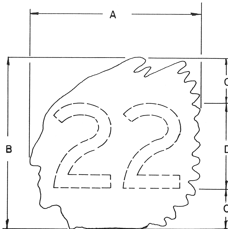
M1-5A STATE ROUTE MARKER (FOR GUIDE SIGN USE)
