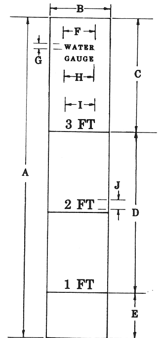
GAUGE BOARD Size 9 X 48
